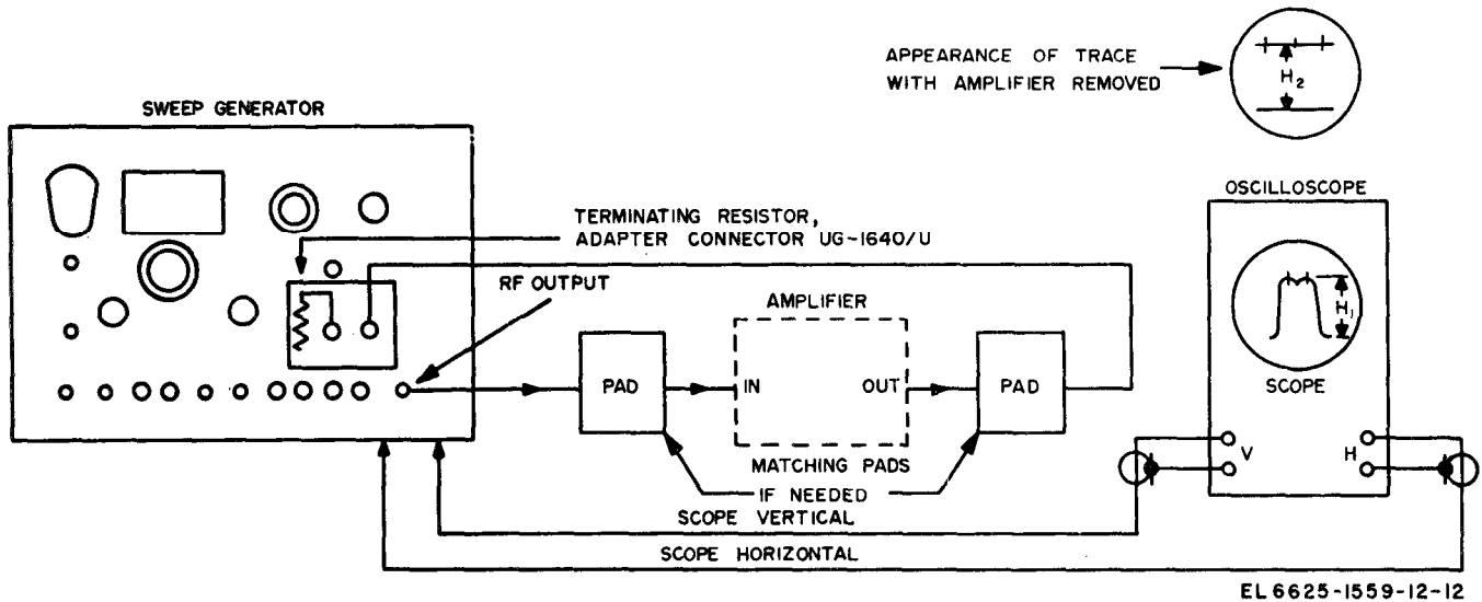
Figure 3-7. Setup for testing RF amplifier.
