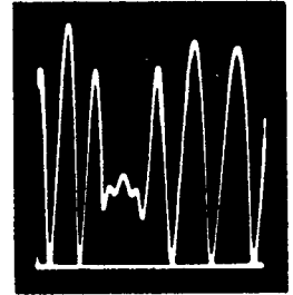
E. RESPONSE CURVE WITH A TERMINATION MATCHING ONLY A NARROW SECTION OF THE SWEEP BAND.
