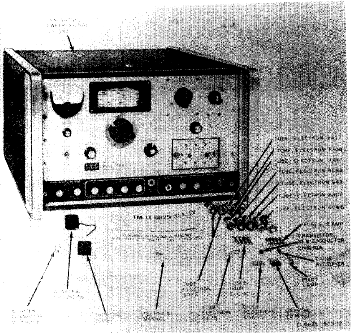
Figure 1-1. Generator, Signal Sweep AN/USM-203.
