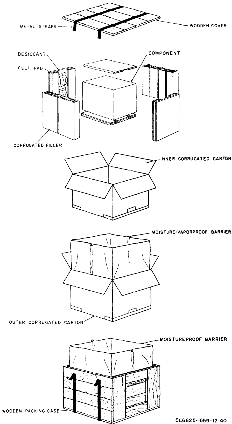
Figure 2-1. AN/USM-203 packaging.
