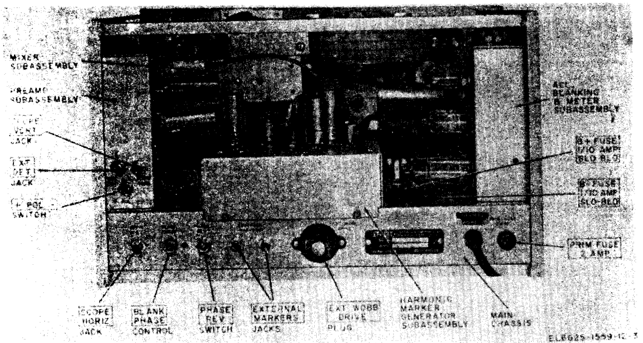
Figure 1-3. Generator, Signal Sweep SG-593/U, rear view.
