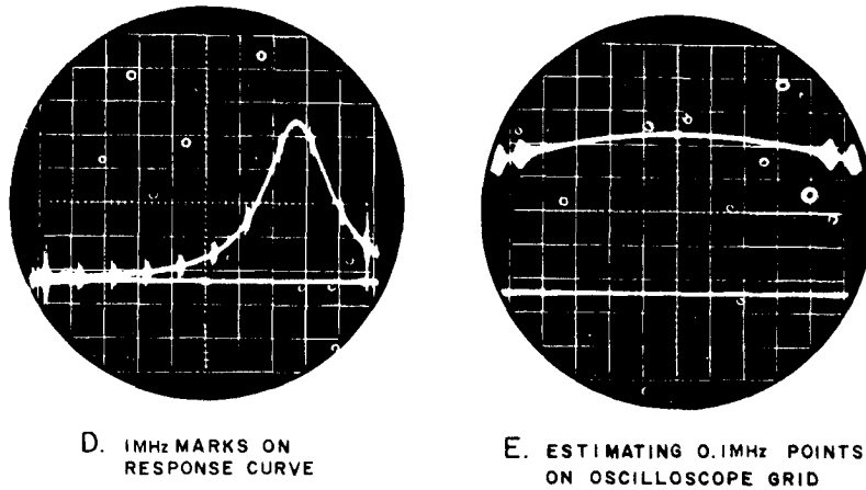
Figure 3-2. Typical oscilloscope display using internal markers.
